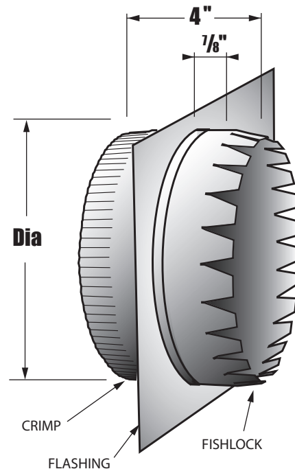
Starter Collar Connector Duct Board
